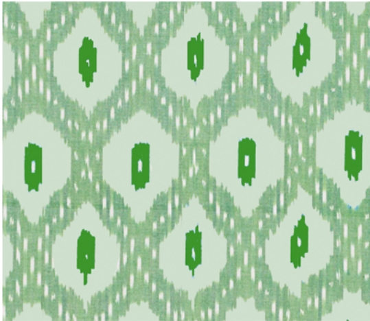
1. monochromatic
